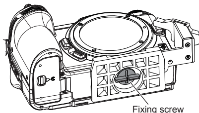
Fixing screw
