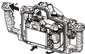
Fixing screw
